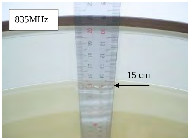
Fig.2.1 Photograph of the Tissue Simulant Fluid liquid depth 15cm for Flat position
