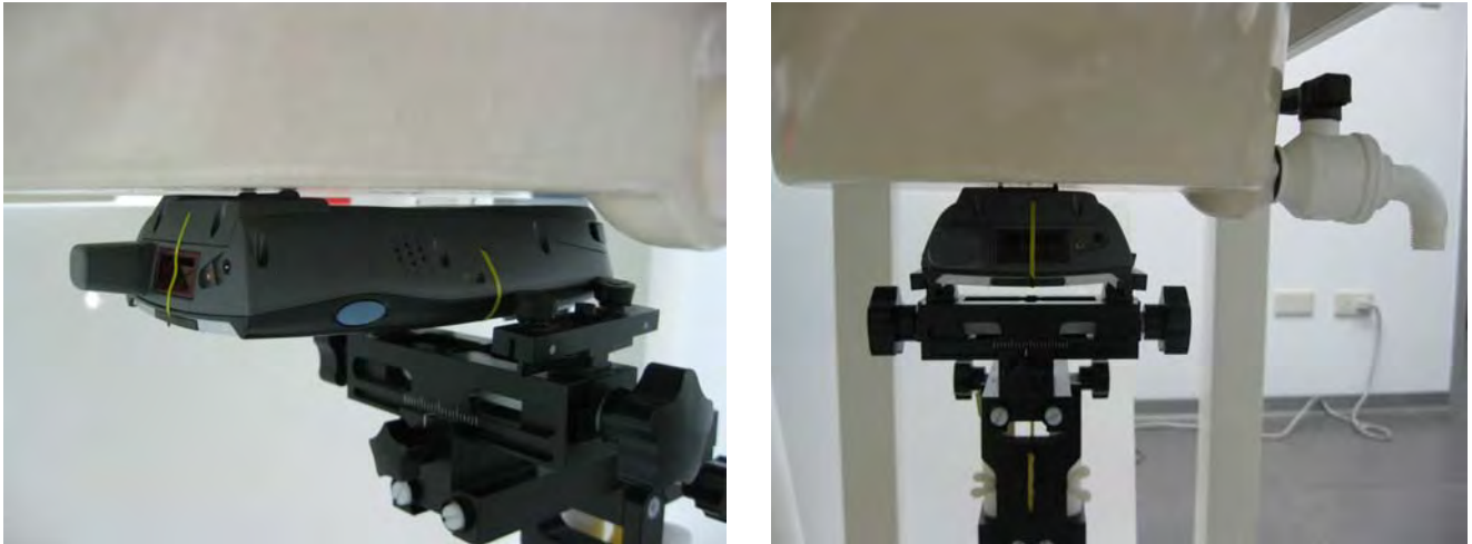
Fig.3.2 back side of EUT is paralleled with flat phantom, separating 0cm between the back of the EUT and the flat phantom.
