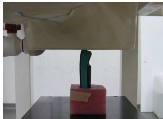
Fig.10 EUT Top side to flat phantom
