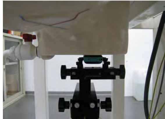
Fig.8 EUT Front side mode to flat phantom
