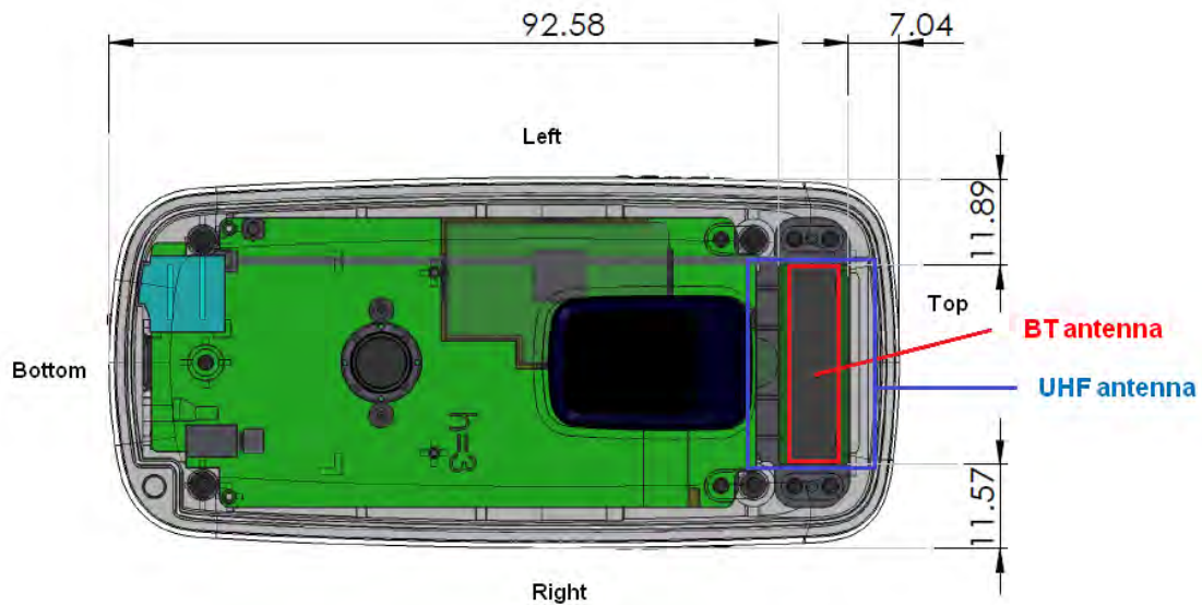
Fig.15 Antenna location (front view)
