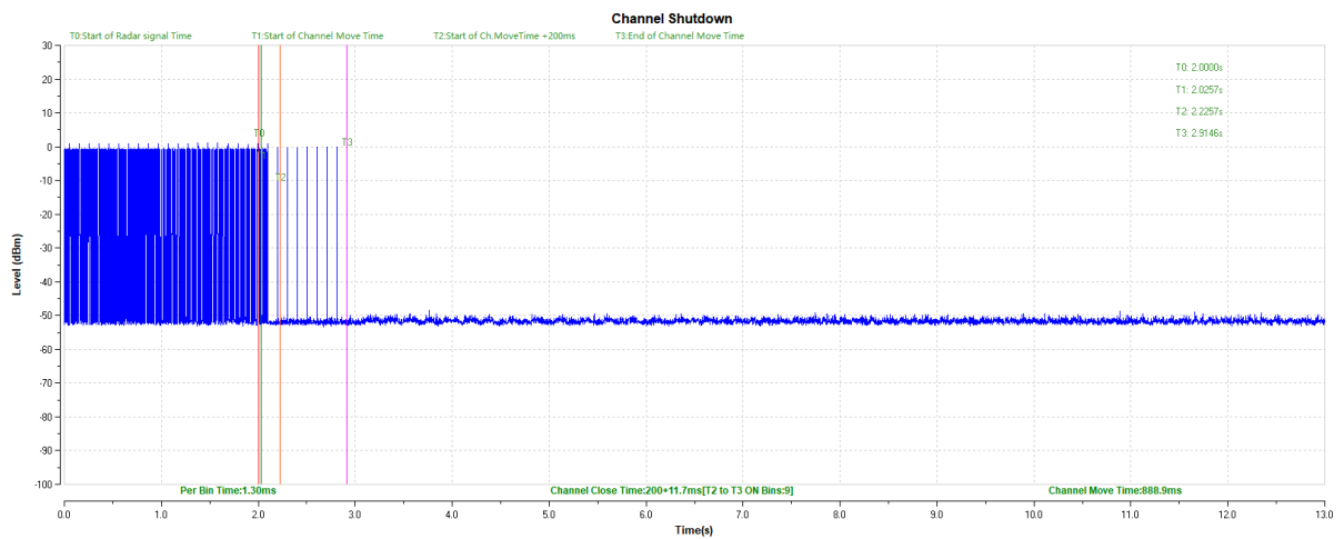
Fig.1 Channel Shutdown (HT20 Frequency Band: 5250MHz ~ 5350MHz)
