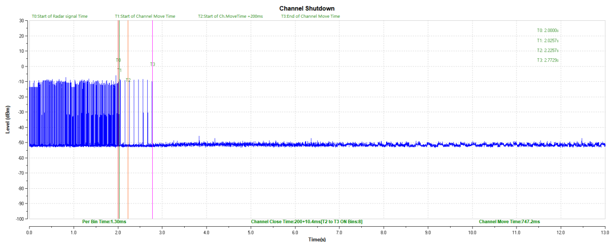
Fig.2 Channel Shutdown (HE160 Frequency Band: 5470MHz ~ 5725MHz)
