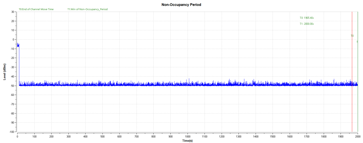
Fig.4 Non-Occupancy Period (HE160 Frequency Band: 5470MHz ~ 5725MHz)
