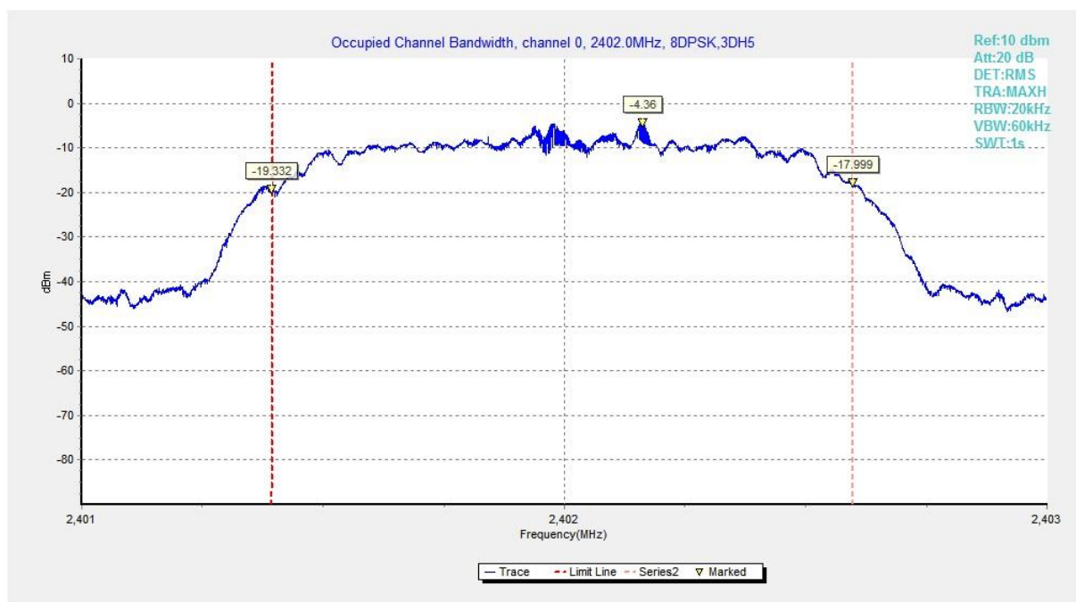
Fig. 83 99% Occupied Bandwidth (8DPSK, Ch 0)
