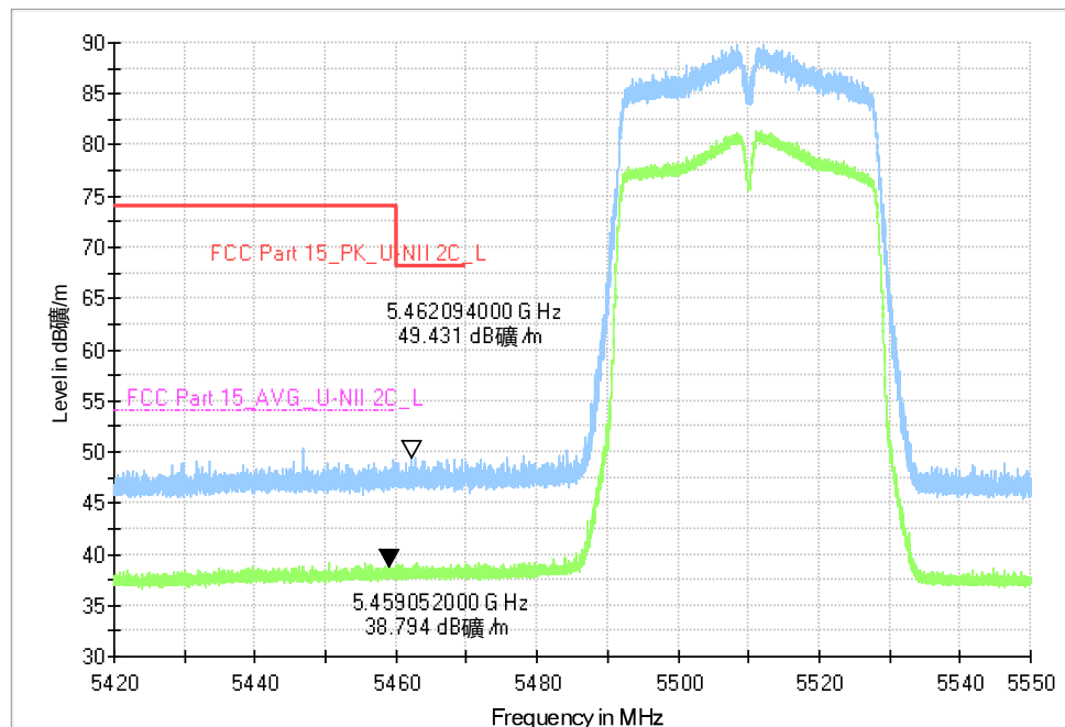
Fig. 61 Band Edges (802.11n-HT40, CH102 5510MHz)
