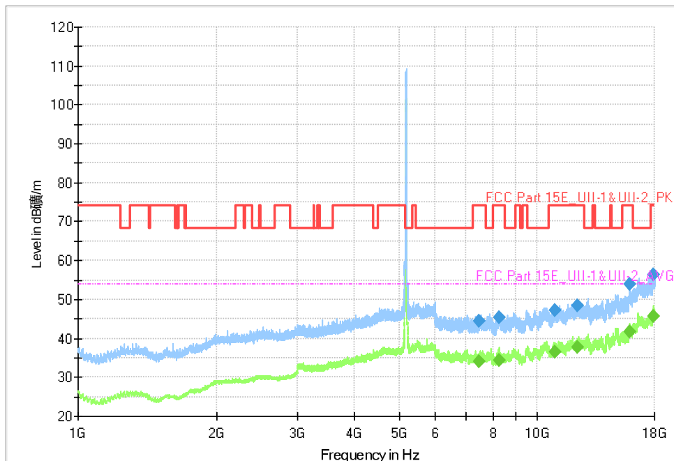
Fig. 71 Transmitter Spurious Emission (802.11a, CH36 5180MHz)
