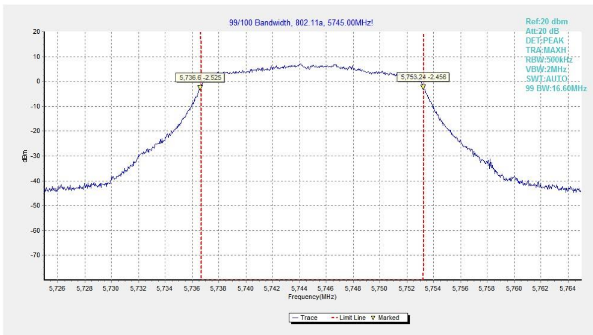
Fig. 36 99% Occupied Bandwidth (802.11a, 5745MHz)
