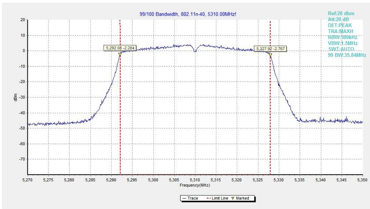
Fig. 42 99% Occupied Bandwidth (802.11n-HT40, 5310MHz)
