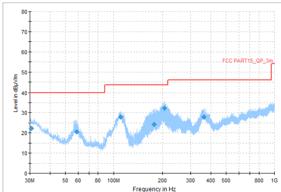
Fig. 97 Transmitter Spurious Emission (All channel, 30MHz~1GHz)
