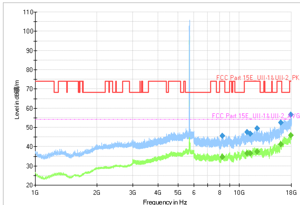
Fig. 79 Transmitter Spurious Emission (802.11a, CH140 5700MHz)
