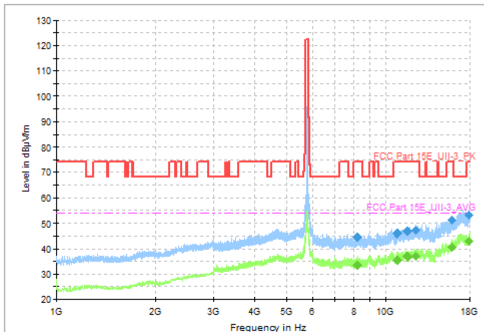
Fig. 94 Transmitter Spurious Emission (802.11ac-VHT80, CH155 5775MHz)
