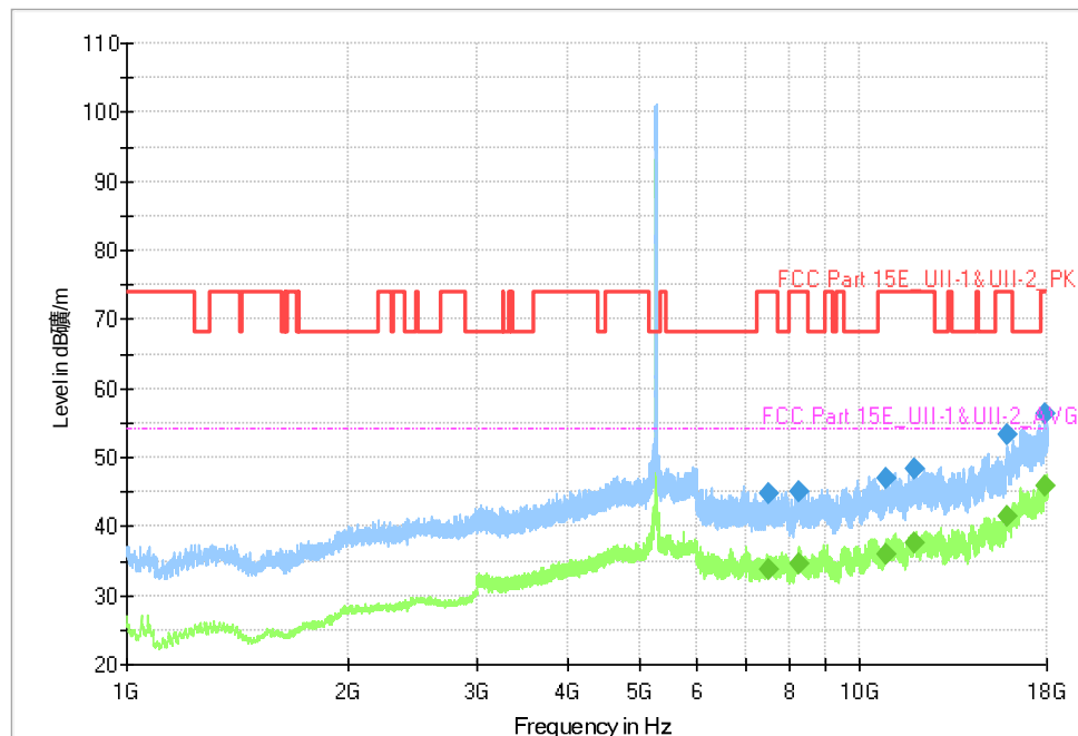
Fig. 85 Transmitter Spurious Emission (802.11n-HT40, CH54 5270MHz)
