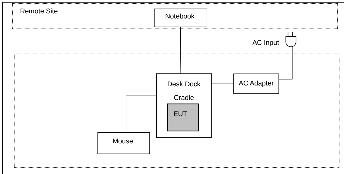
Radiated Emissions
