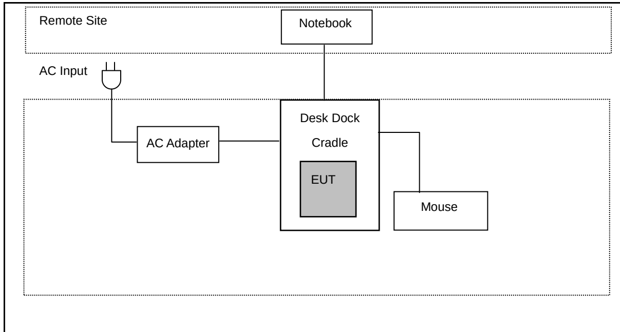
AC Power Conducted Emission
