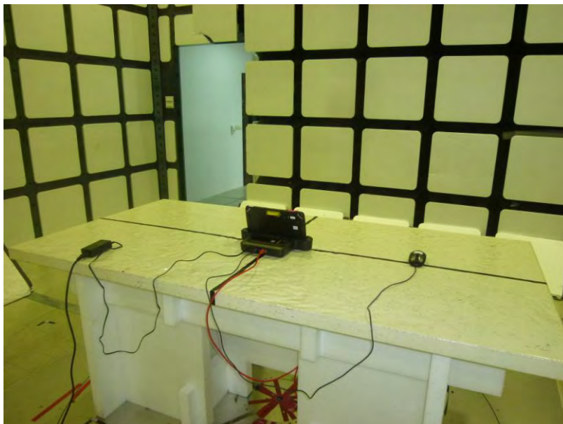
30MHz ~ 1GHz _ Rear View
