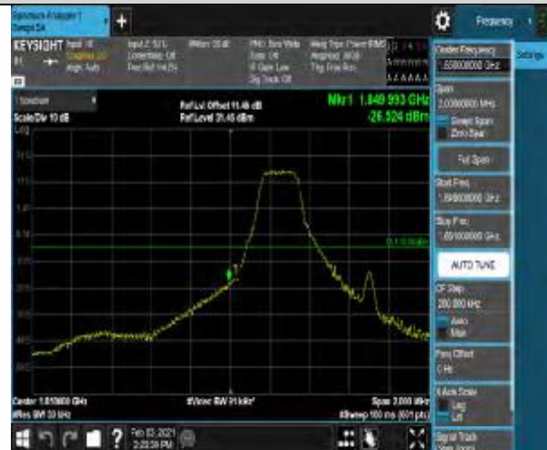
Band2-1.4MHz-64QAM-18607-1RB#5
