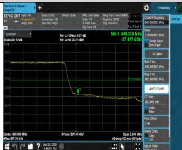
Band26-1.4MHz-16QAM-26797-1RB#0
