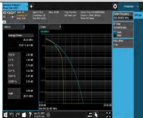
Band26-10MHz-16QAM-26915-50RB#0
