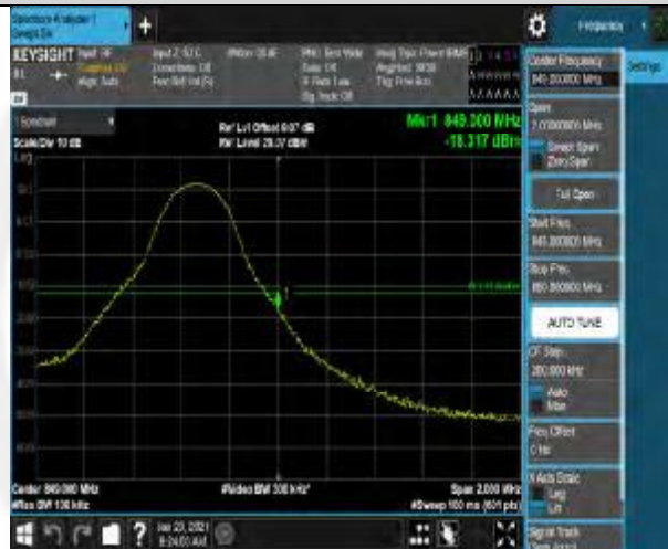
Band26-5MHz-16QAM-27015-25RB#0
