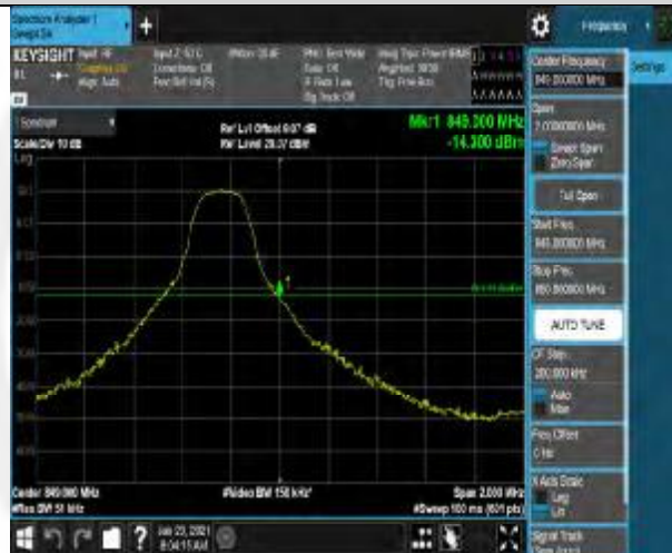
Band26-3MHz-QPSK-27025-15RB#0
