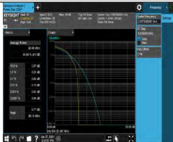
Band41-5MHz-16QAM-41565-25RB#0
