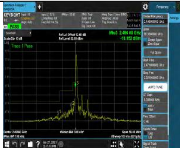
Band41-5MHz-QPSK-39675-1RB#24
