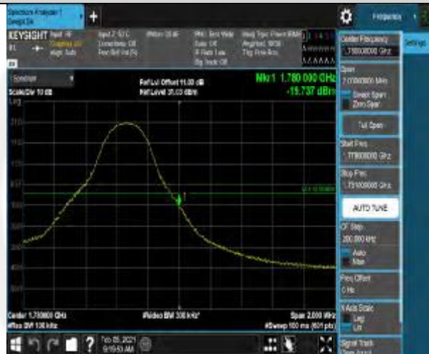
Band66-5MHz-64QAM-132647-25RB#0
