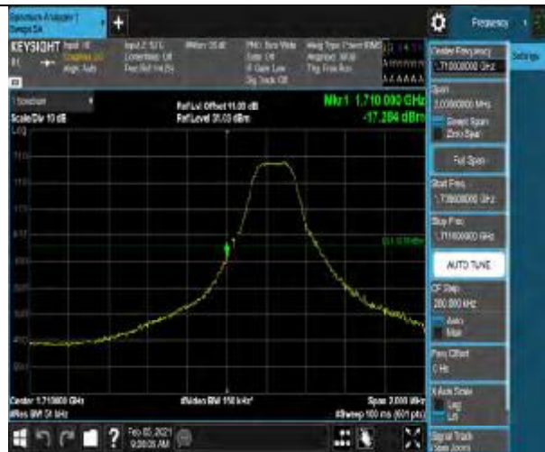
Band66-3MHz-64QAM-131987-1RB#14
