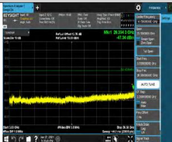
Band41-10MHz-16QAM-39700-1RB#0-Range3:3000~26500MHz
