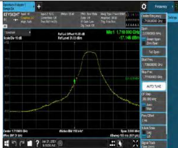
Band66-3MHz-QPSK-131987-1RB#14
