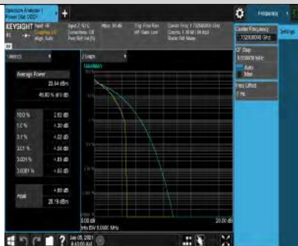
Band4-3MHz-QPSK-20175-15RB#0
