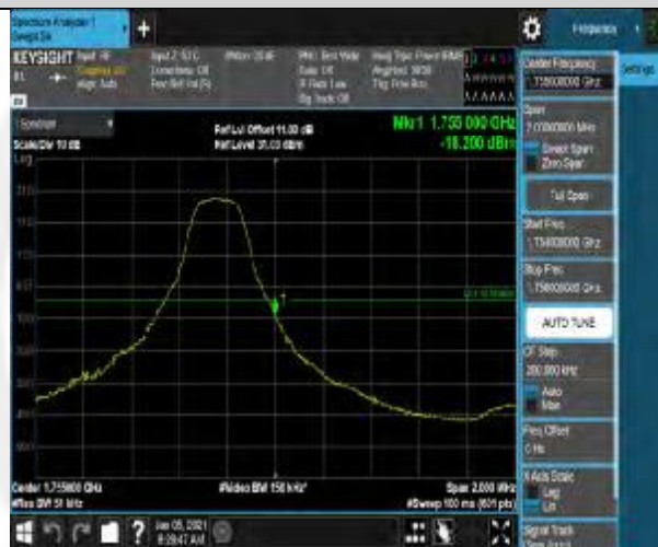
Band4-3MHz-QPSK-20385-15RB#0
