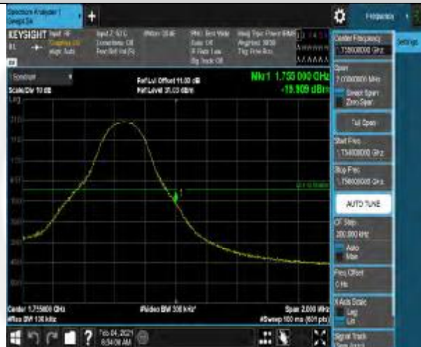
Band4-5MHz-64QAM-20375-25RB#0
