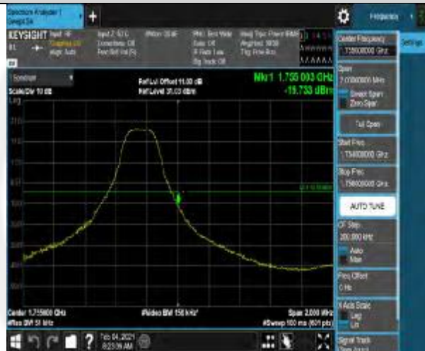
Band4-3MHz-64QAM-20385-15RB#0
