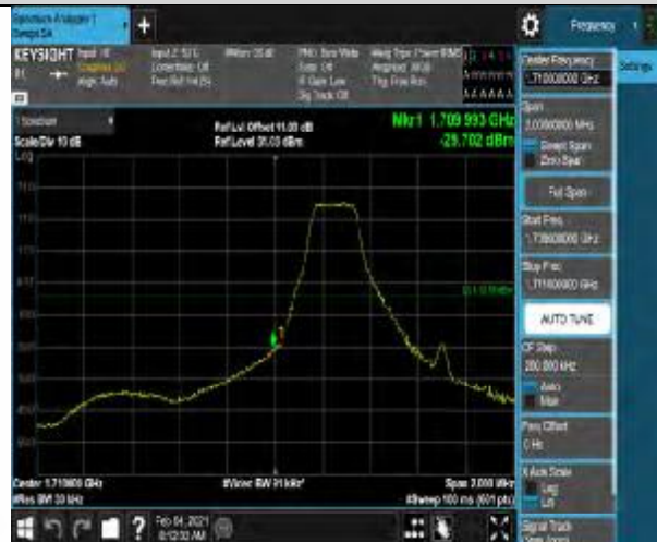
Band4-1.4MHz-64QAM-19957-1RB#5
