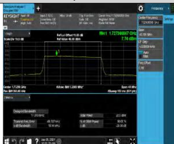
Band4-20MHz-16QAM-20300-100RB#0-17.971
