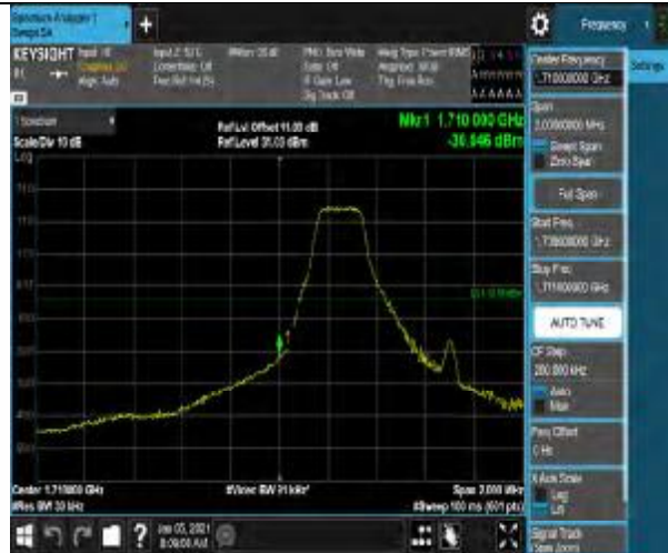
Band4-1.4MHz-16QAM-19957-1RB#5
