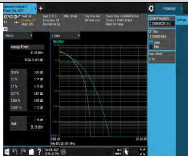
Band7-15MHz-64QAM-20825-1RB#0
