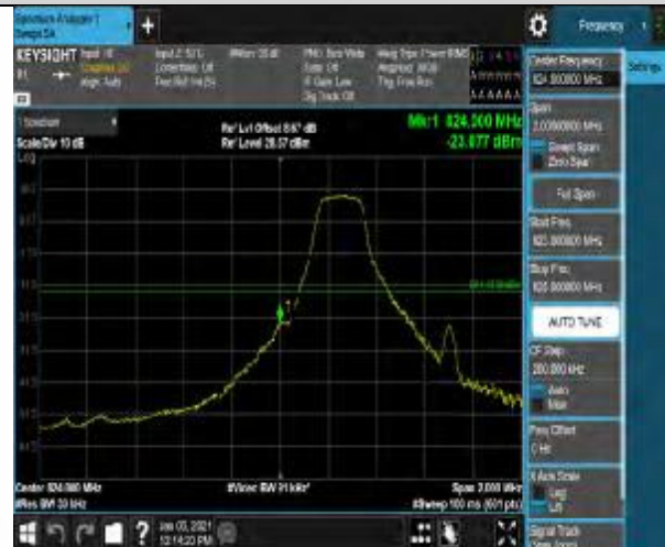
Band5-1.4MHz-QPSK-20407-1RB#5
