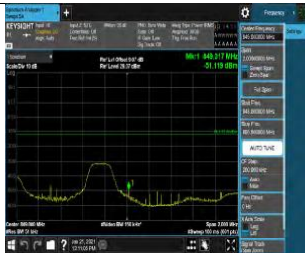
Band5-3MHz-16QAM-20635-1RB#14
