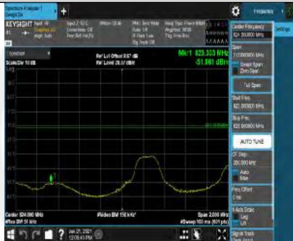
Band5-3MHz-16QAM-20415-15RB#0
