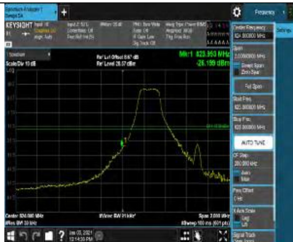
Band5-1.4MHz-16QAM-20407-1RB#5
