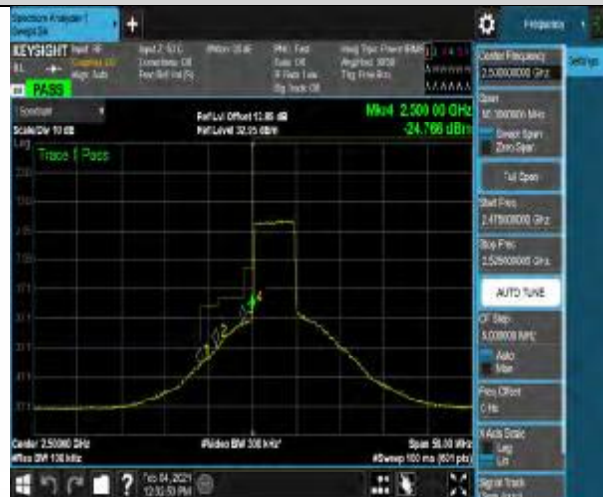
Band7-5MHz-64QAM-20775-25RB#0
