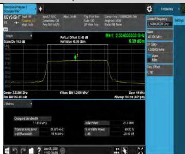
Band7-20MHz-QPSK-21350-100RB#0-17.933
