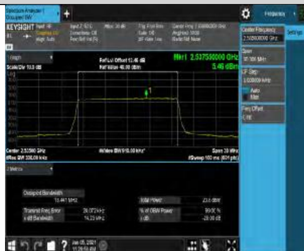
Band7-15MHz-16QAM-21375-75RB#0-13.464
