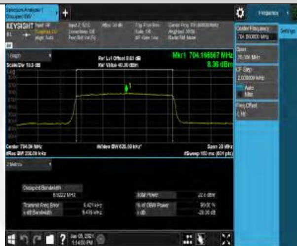
Band12-10MHz-16QAM-23095-50RB#0-8.9914
