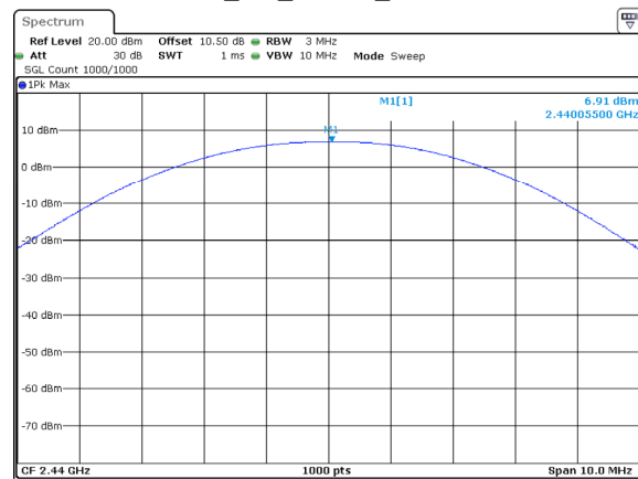
BLE_1M_Middle_Channel
