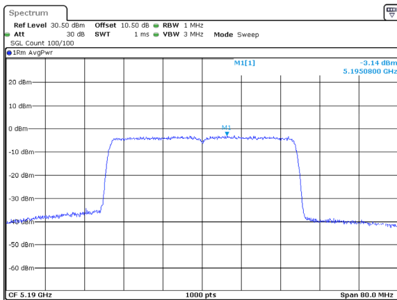
802.11ax40_5190MHz_RU_Full_ANT2
