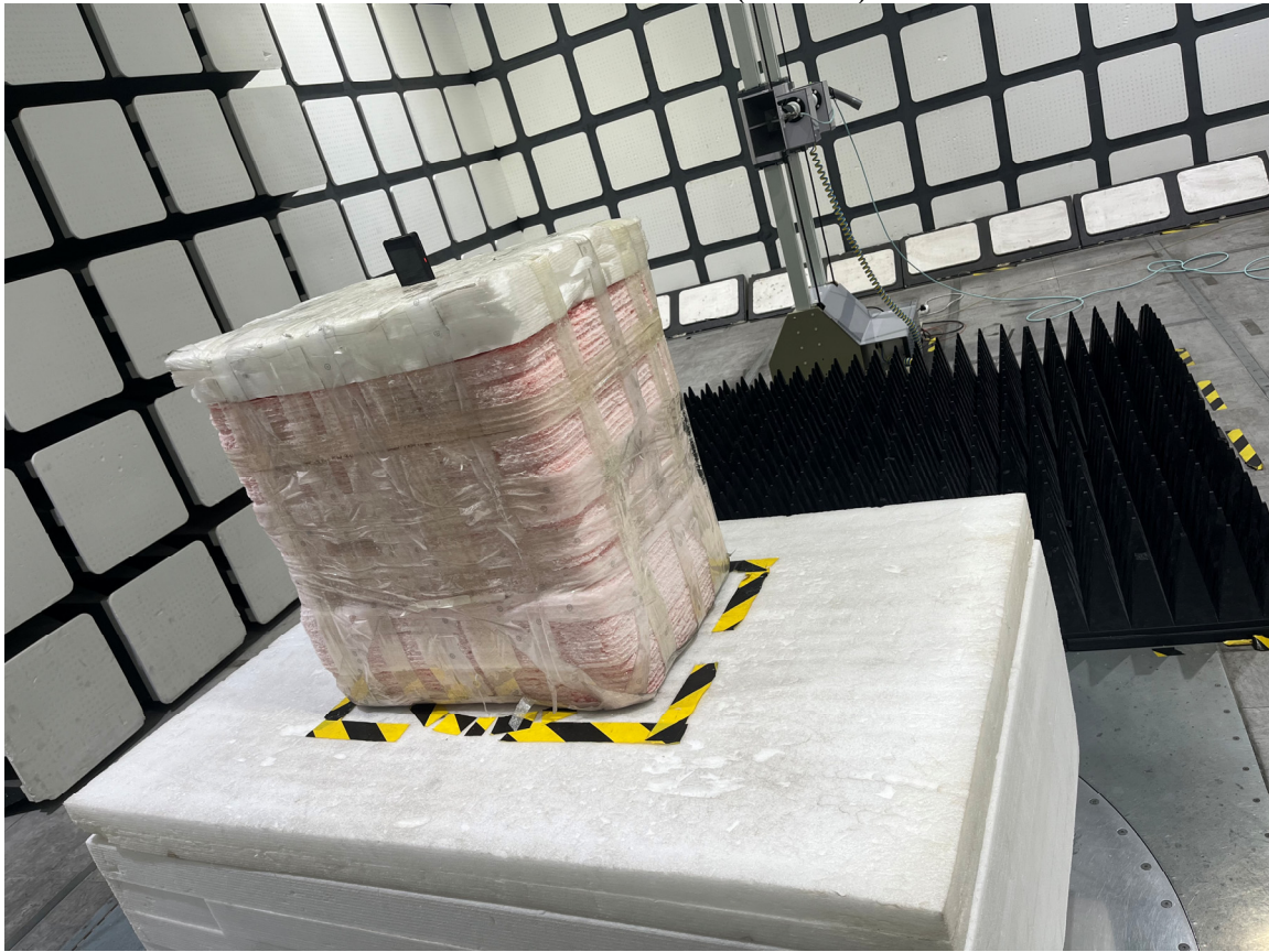
Radiated Emissions View (1-18GHz)
