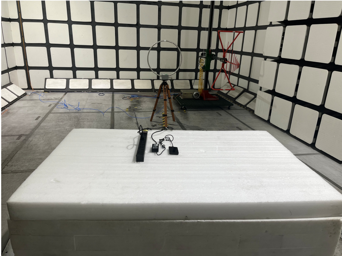
Radiated Emissions View (Below 30MHz)
