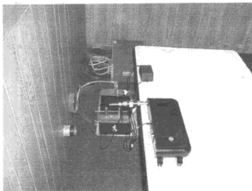
PHOTOGRAPHS 1 & 2: CONDUCTED EMISSIONS TEST SETUP
