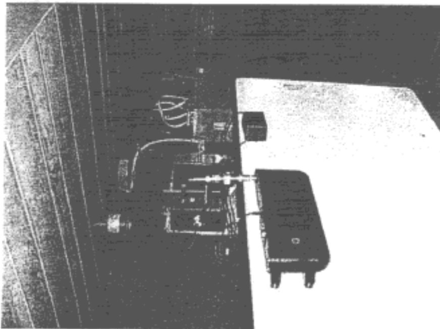
PHOTOGRAPHS 1 & 2: CONDUCTED EMISSIONS TEST SETUP
