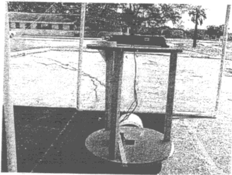
PHOTOGRAPHS 3 & 4: RADIATED EMISSIONS TEST SETUP
