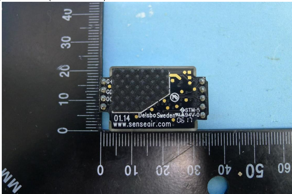
(20) EUT Photo(CO2 Sensor)
