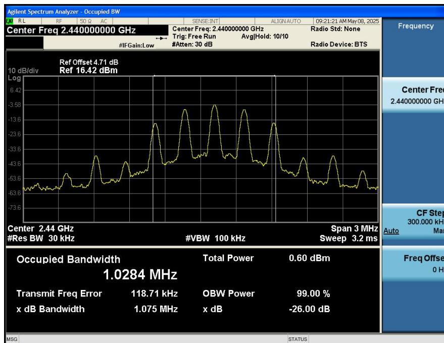
99%_Occupied_Bandwidth_NVNT_ANT1_2.4G_2440_00
