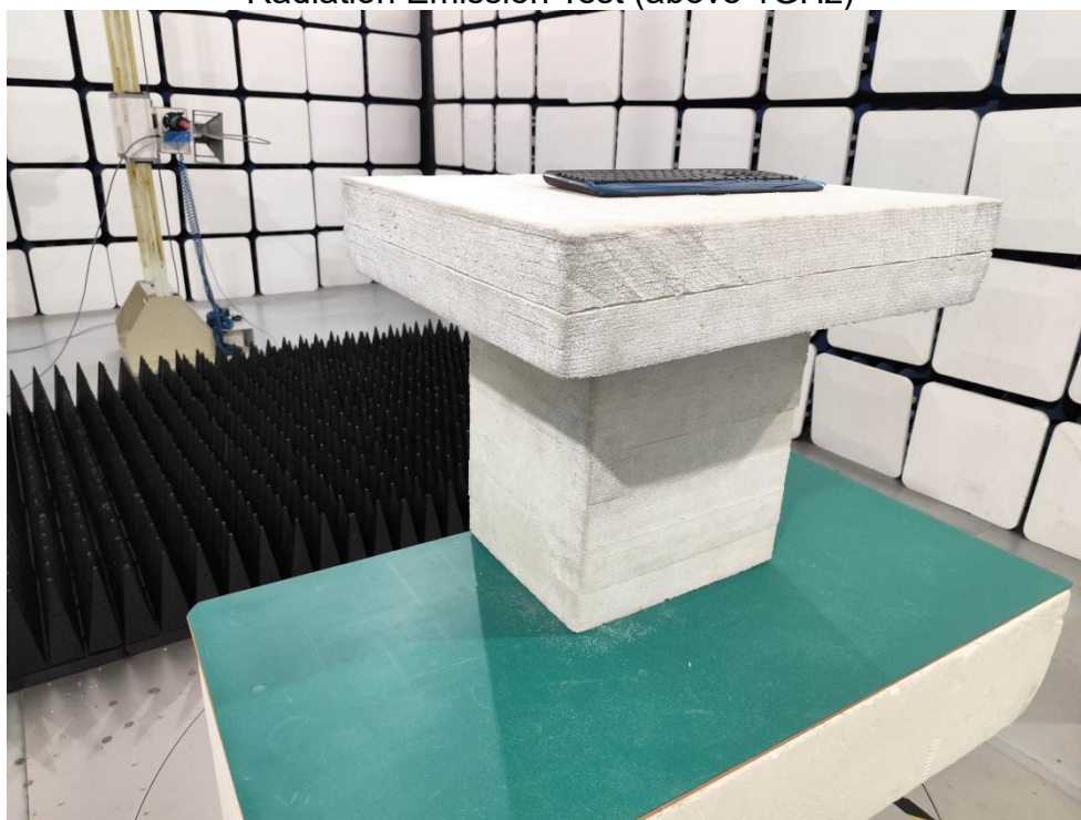
Radiation Emission Test (above 1GHz)
