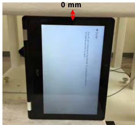
Fig.6 EUT Left side to flat phantom
