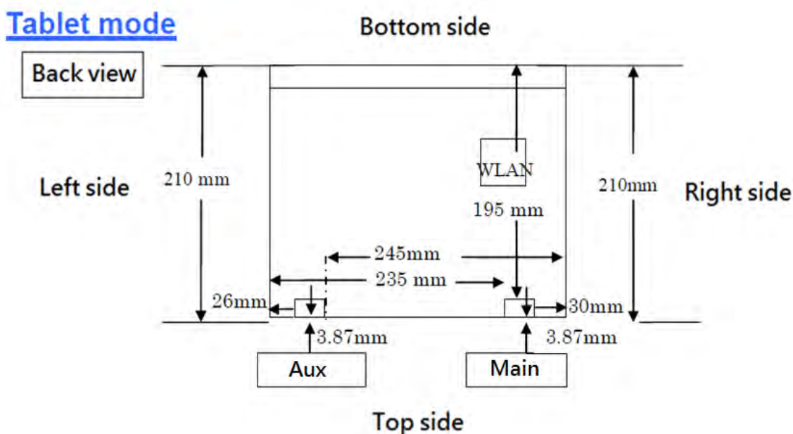
Fig.10 Antenna position of EUT (Back view)
