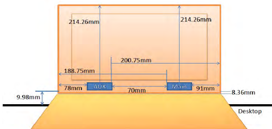
Antenna location
