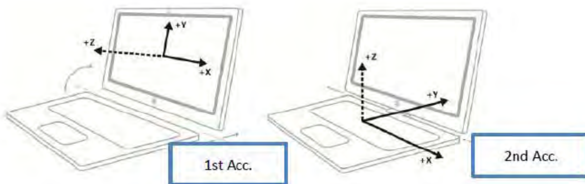
Fig.15 G-sensor location definition
