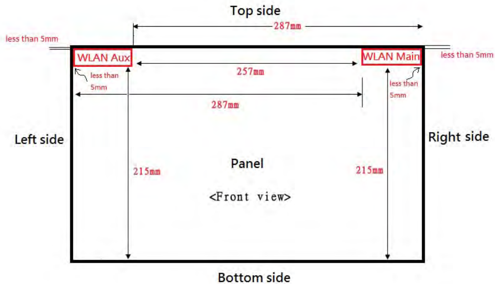
Fig.11 Antenna location of EUT (tablet mode)
