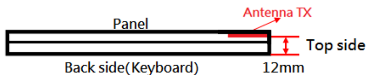
Fig.13 Antenna location of EUT (laptop mode)
