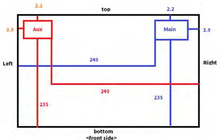
Antenna location
