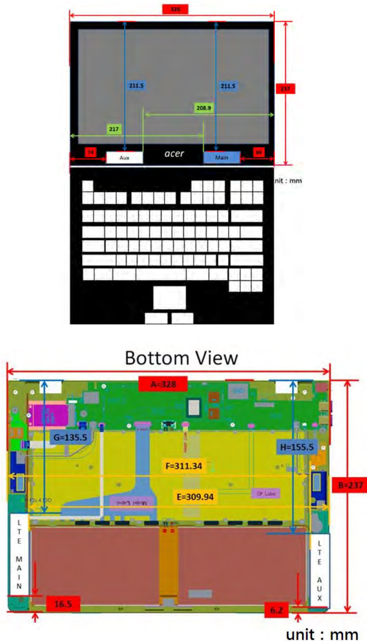
Fig.7 Antenna position of EUT
