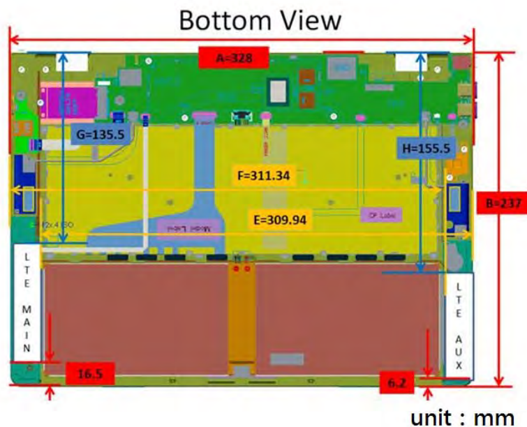
Fig.7 Antenna position of EUT
