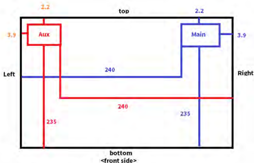
Fig.10 Antenna position of EUT
