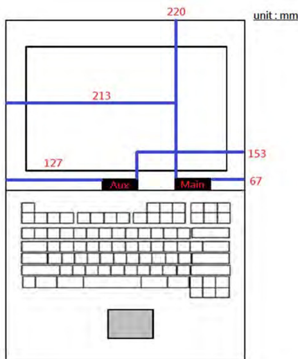
Antenna location
