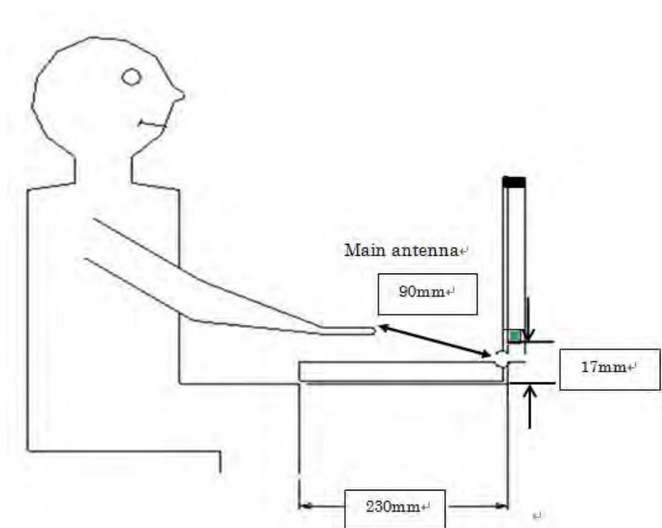
Antenna location (laptop mode)
