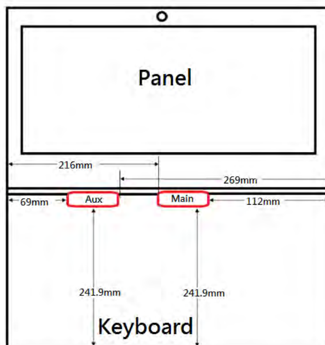
Antenna location (laptop mode)
