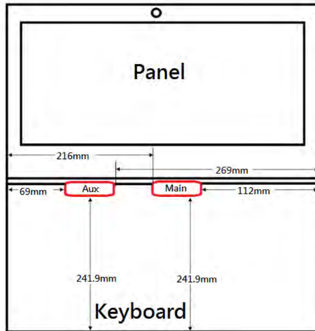
Fig.6 Antenna position of EUT (laptop mode)
