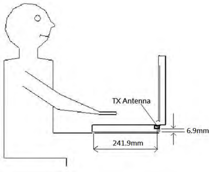
Fig.6 Antenna position of EUT (laptop mode)
