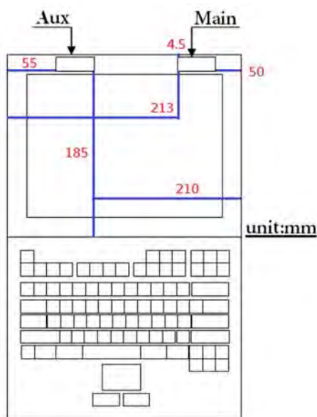
Fig.7 Antenna location (front view of laptop mode)
