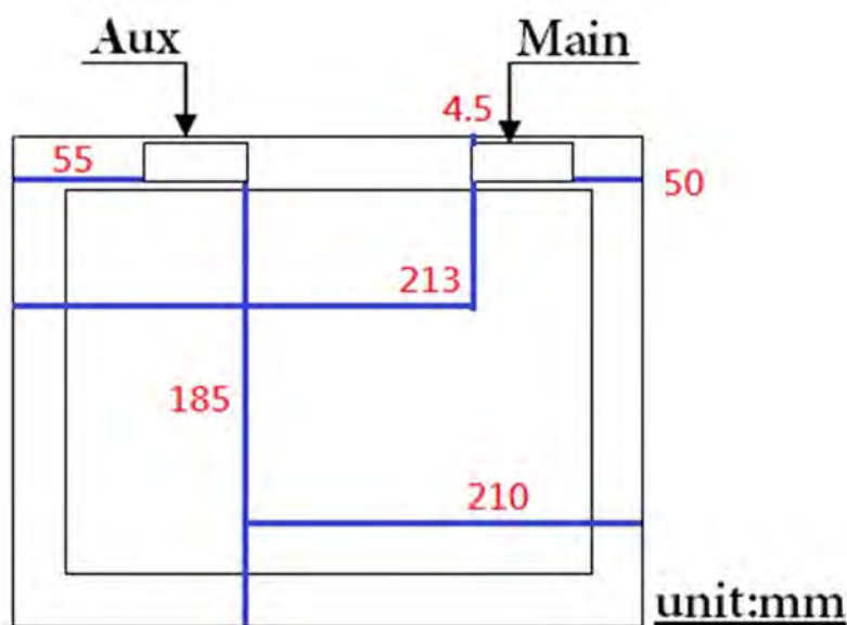
Fig.8 Antenna location (front view of tablet mode)
