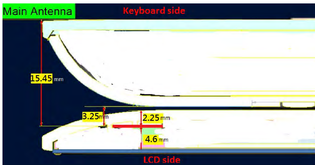
Fig.9 Antenna location (edge view of tablet mode)
