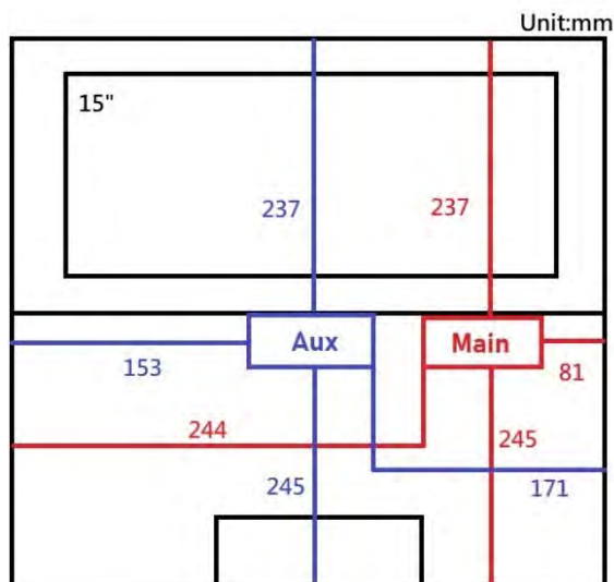
Fig.6 Antenna location (front view of laptop mode)
