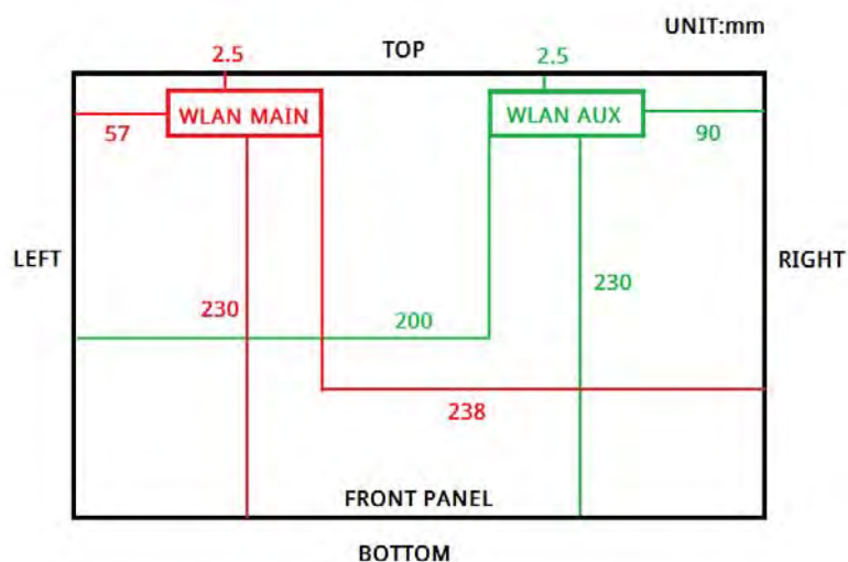
Fig.10 Antenna location of EUT
