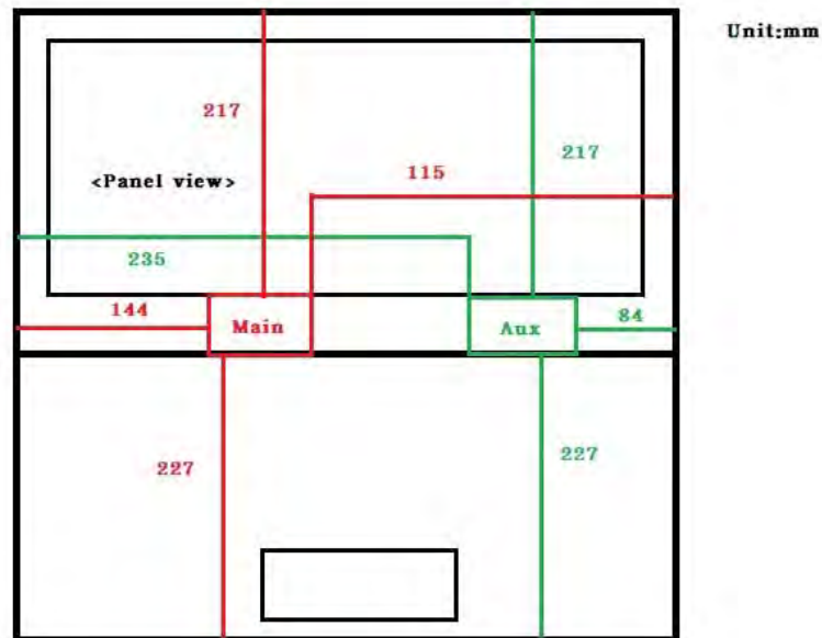
Fig.6 Antenna position of EUT
