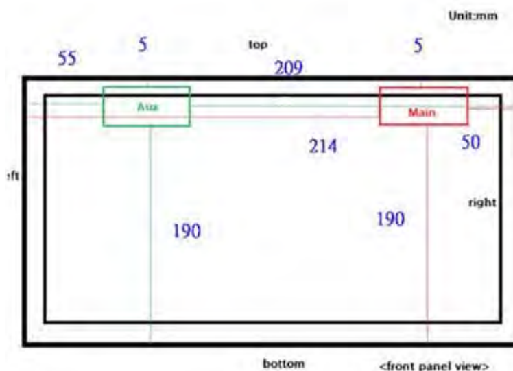
Fig.10 Antenna location of EUT
