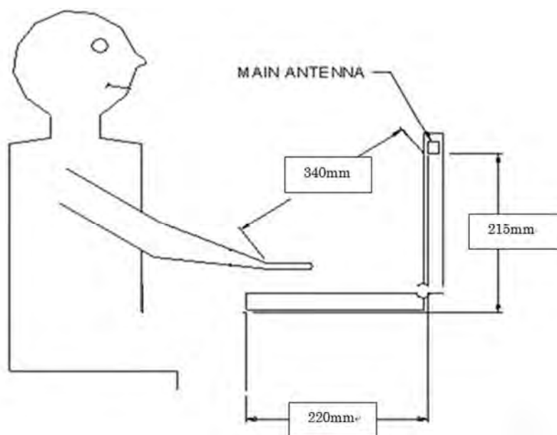
Fig.13 Antenna location of EUT (laptop mode)
