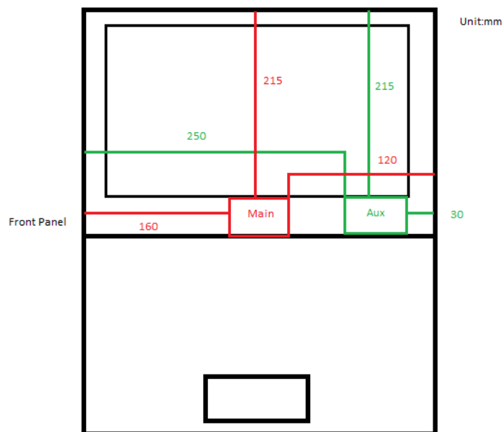
Fig.6 Antenna location of EUT (laptop mode)
