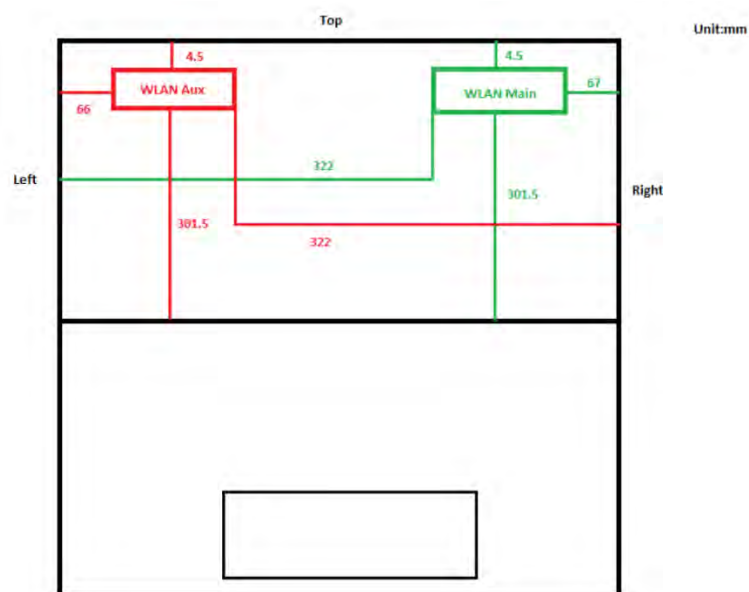
Fig.14 Antenna location of EUT (Notebook mode)
