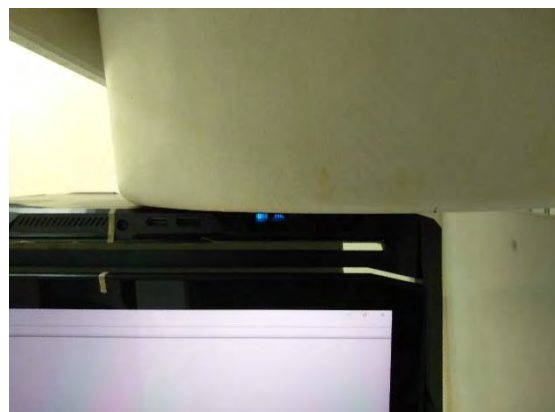
Fig.8 EUT Bottom side (Display Mode_Main) to flat phantom
