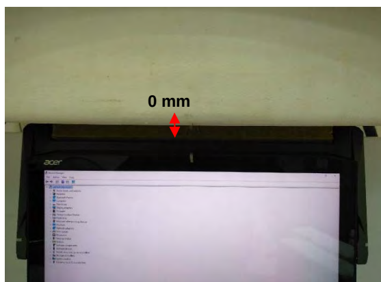
Fig.4 EUT Top side (Stand Mode) to flat phantom
