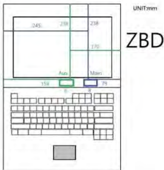
Fig.6 Antenna location of EUT
