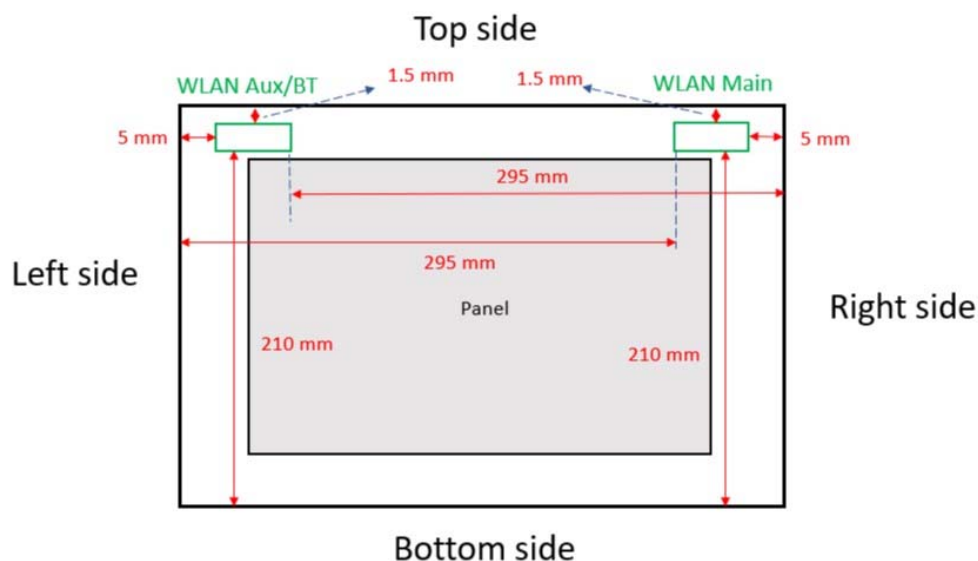
Fig.9 Antenna location of EUT (Tablet mode)
