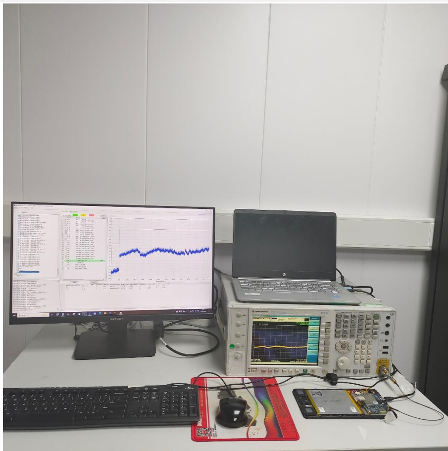
Conducted Test-BT/WIFI
