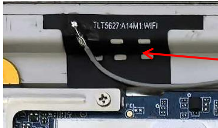
WIFI Antenna
