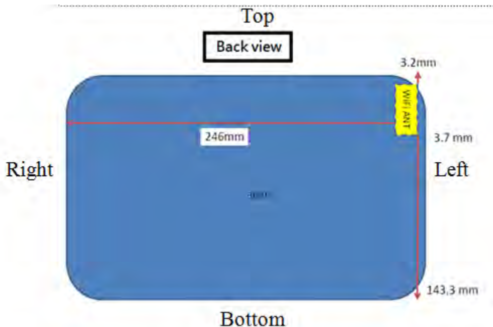
Fig.8 Antenna position of EUT (Back view)
