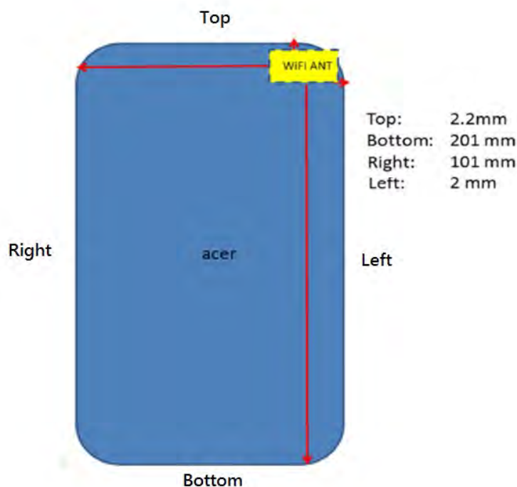
Fig.9 Antenna position of EUT (Back view)
