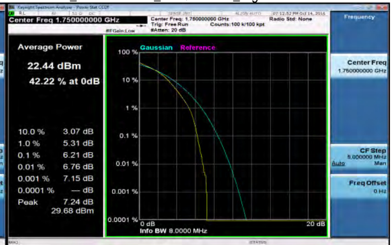
LTE_Band4 10MHz_16-QAM 50 0_HighCH20350-1750
