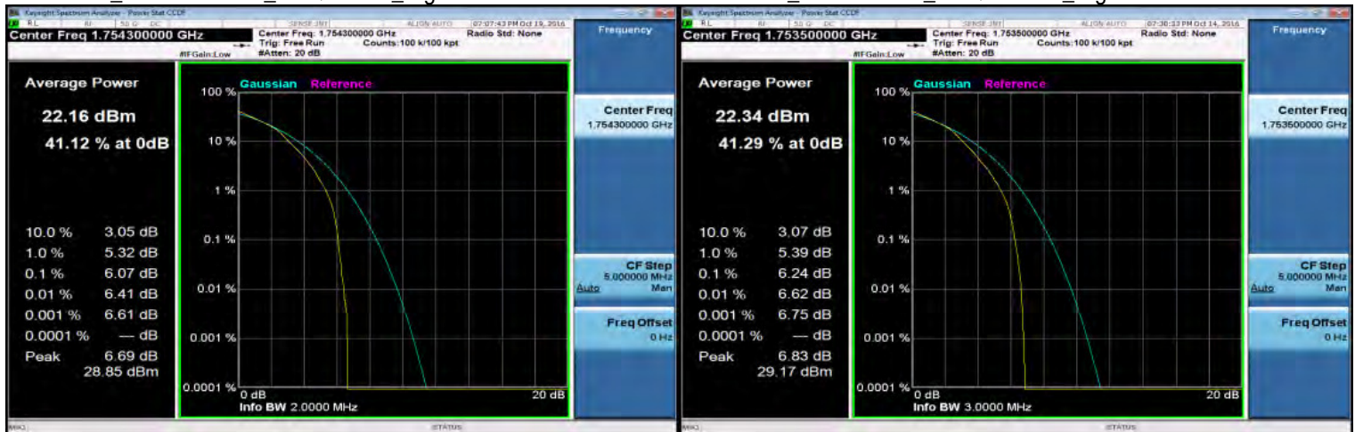
LTE_Band4 1.4MHz_16-QAM 6 0_HighCH20393-1754.3
