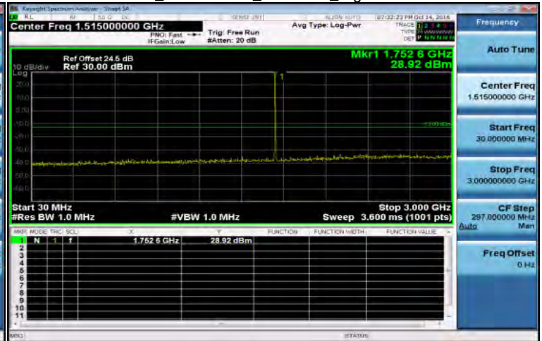
30MHz~3GHz_Band4 3MHz_QPSK 1 0_HighCH20385-1753.5
