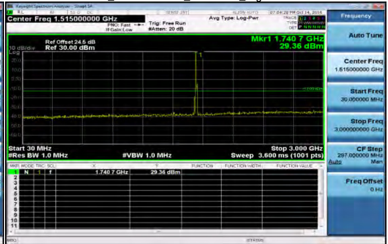
30MHz~3GHz_Band4 15MHz_QPSK 1 0_HighCH20325-1747.5
