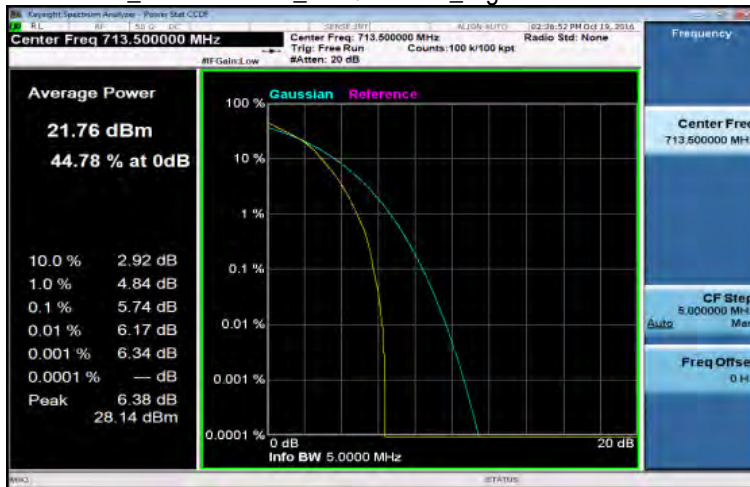
LTE_Band12 5MHz_16-QAM 25 0_HighCH23155-713.5
